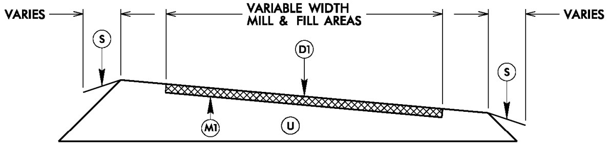
MILL & FILL PATCHING DETAIL
